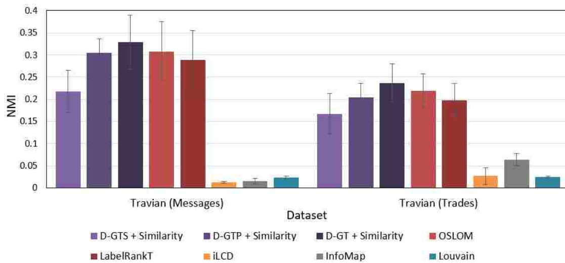
Figure 4.8: Normalized mutual information (NMI) evaluation metric on the two Travian datasets with ground truth community membership information; results are averaged over all snapshots. The variants of D-GT are colored in purple, LabelRankT (red), OSLOM (indian red), iLCD (yellow), InfoMap (gray) and Louvain (blue).
