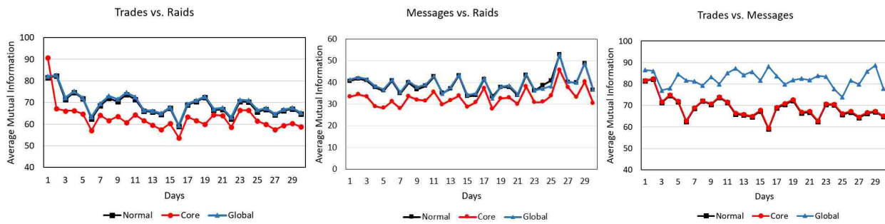
Figure 7.1: Average mutual information values over time calculated using normal and core neighborhood definitions for (a) Travian trades as the target layer and raids as the predictor, (b) Travian messages as the target layer and raids as the predictor, and (c) Travian trades as the target layer and messages as the predictor.
